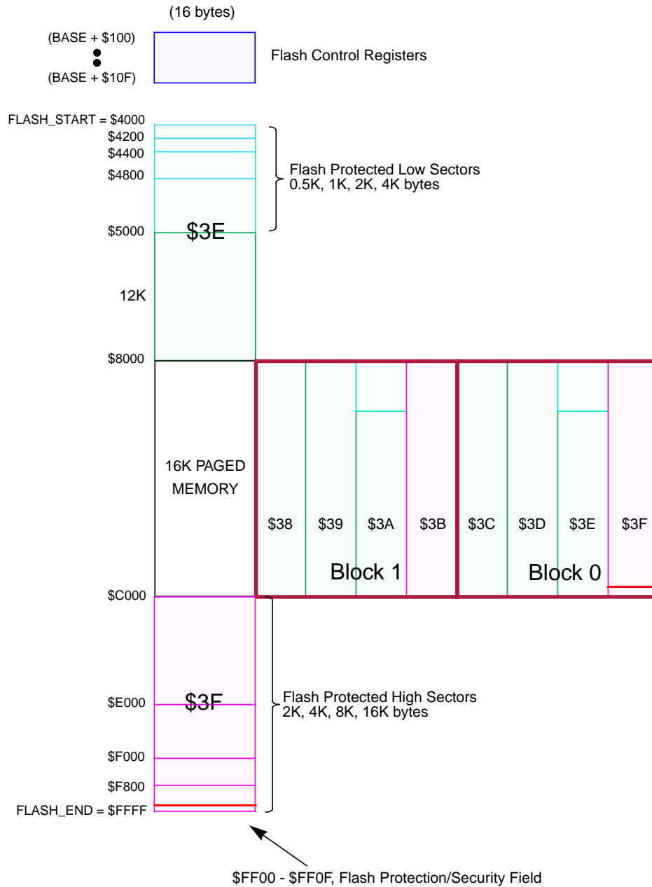
Figure 3-1 FTS128K Flash Memory Map
