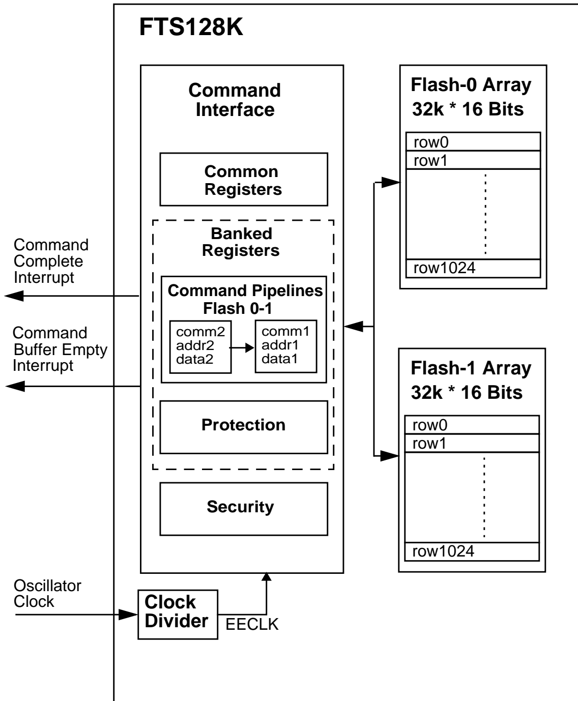
Figure 1-1 FTS128K Module Block Diagram
