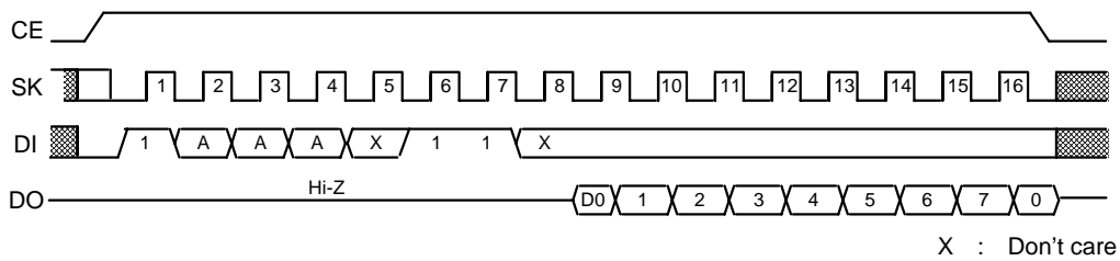
Figure 9 Read mode timing(S-24H30, S-24S30)
