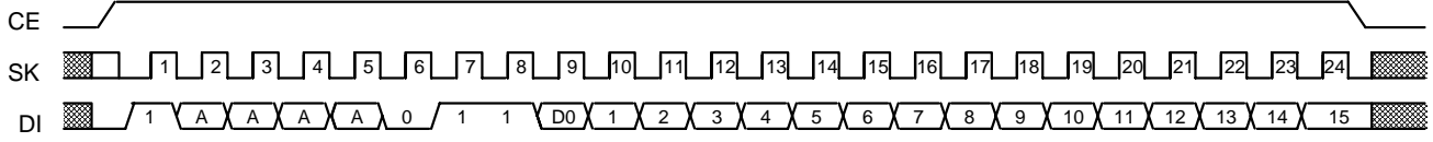
Figure 10 Write mode timing(S-24H45, S-24S45)
